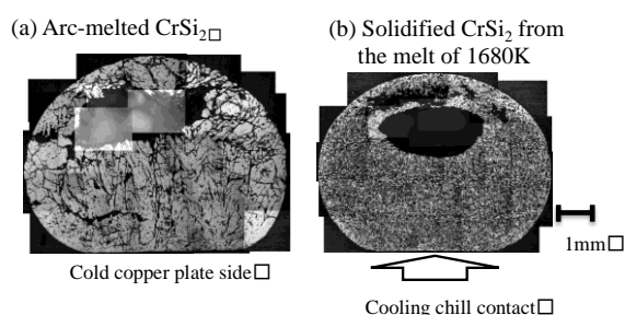
Fig.1 Cross section of CrSi 2 sample solidified from the melt. C
