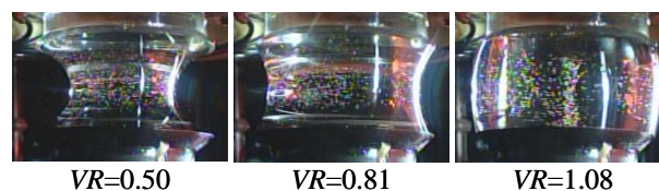
Fig. 1 Shape of liquid bridge for different VR
