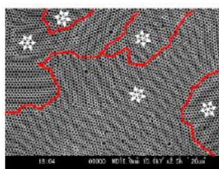
Fig. 2 Domain formation
