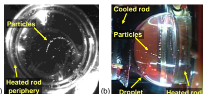
Fig. 1 Example of view obtained by one of the top view cameras (a) and side view camera (b) in on-orbit experiments (MEIS-3)
