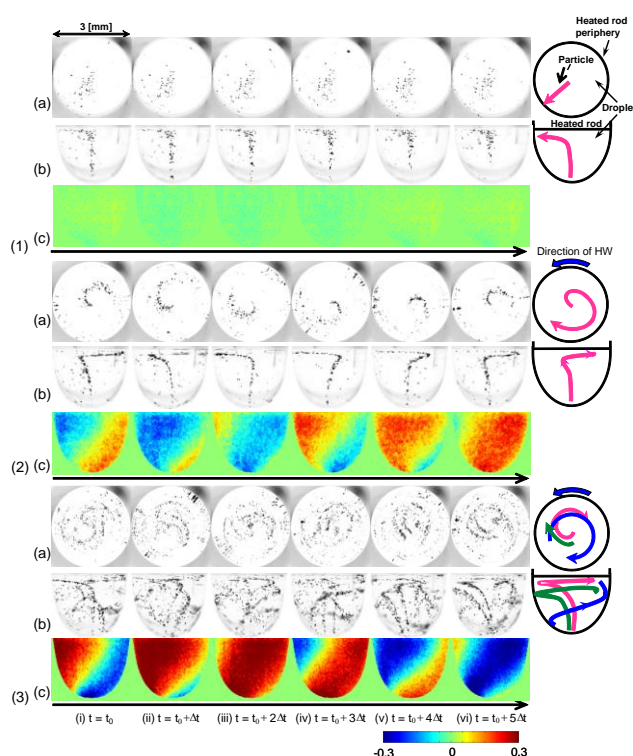
Fig. 2 Time series of snapshots of each flow regimes; (1) Steady flow, (2) Traveling flow, and (3) Dynamic PAS flow at time interval \Delta t [s] of (1) 0.372, (2) 0.178 and (3) 0.117, respectively. Spatio-temporal correlation between particle line observed (a) from above, (b) from side, and (c) the surface temperature deviation observed from another side, respectively. The temperature difference in snapshots of temperature deviation is \pm 0.3 [K]. The HWs of (2) the Traveling wave and (3) the Dynamic PAS flow propagate from the left to the right in the frame (i.e., counterclockwise) in these cases. Schematic views are drawn aside the last image of particle lines. Outer circle in the top view corresponds to the periphery of the top rod whose radius is 1.5 mm.
