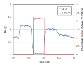
Fig. 4 Control of the illumination of UV lamp.
