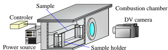
Fig.1 Experimental setup.
