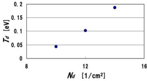
Fig.4 Plot of particle-motion temperature against particle density.
